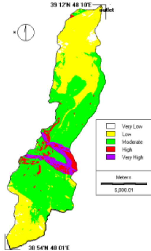
Fig. 2. Landslides hazard zonation map in AHP method
