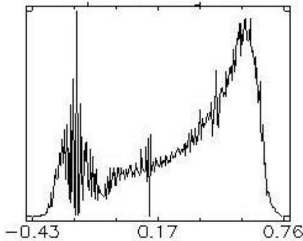
Figure 5 NDVI histogram on 2002 image after normalized to 1995 image
