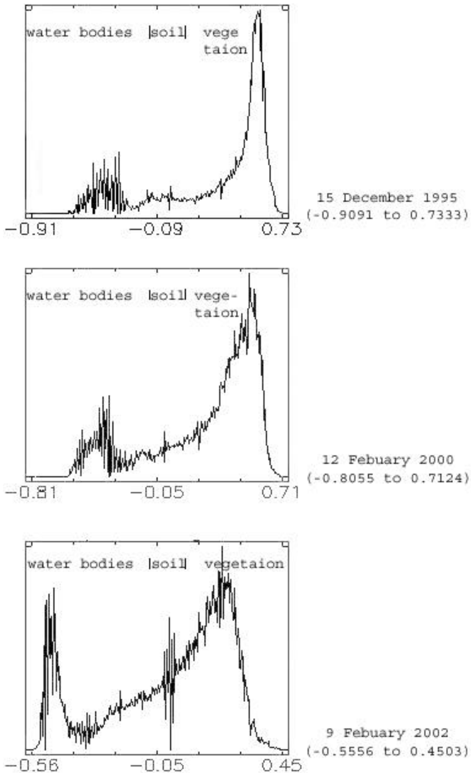
Figure 3 NDVI histogram calculated from 1995, 2000 and 2002 imagery
