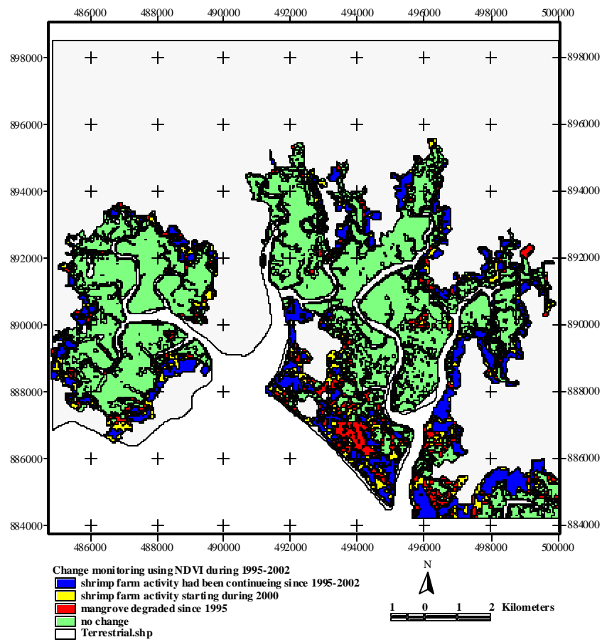
Figure 6 Changes monitoring during 1995-2002 using NDVI
