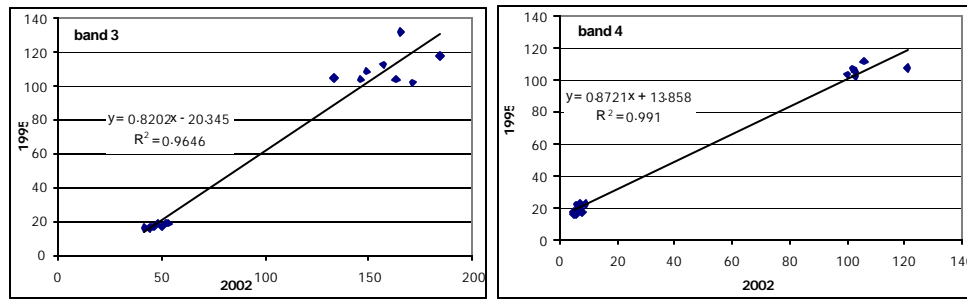
Figure 4 Radiometric correction of LANDSAT (ETM+) data set band 3 and band 4
