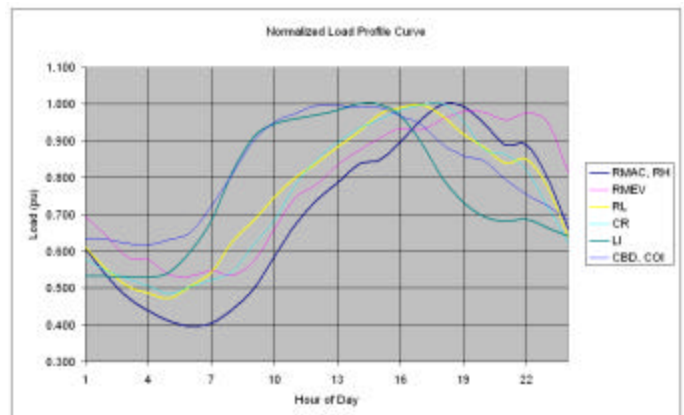
Figure 1: Example of final load curves used.
